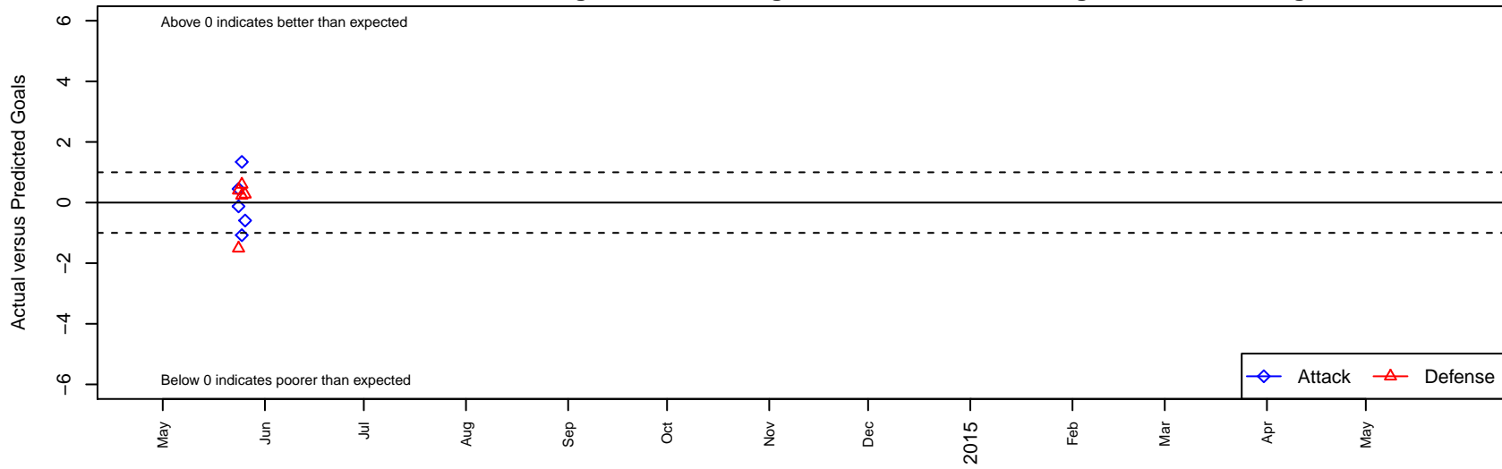
GPYSC Rebels Blue B02 Dots are actual minus expected GF (blue circles) and GA (red triangles). Blue line is smoothed change in attack strength. Red is smoothed change in defense strength.
